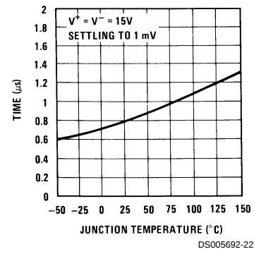
“Hold” Settling Time (Note 10)
