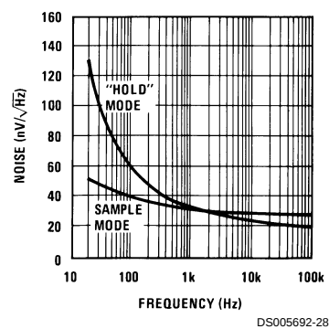
Output Noise
